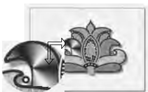
Fast Preview
