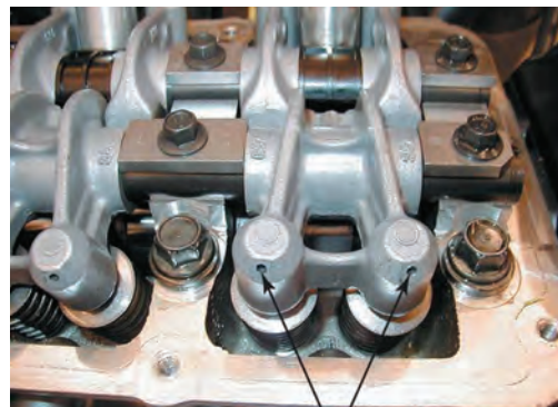
BLEED HOLES FROM HYDRAULIC LASH ADJUSTERS (HLA)
